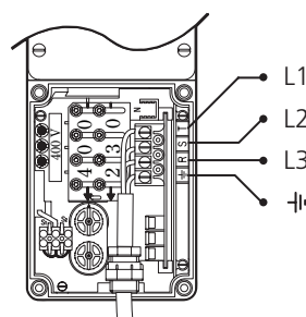
Power supply wiring
