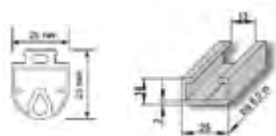
Banda Resistiva SECUBAND 25 SECUBAND 25 resistive band Bande résistive SECUBAND 25 Banda Resistiva SECUBAND 25
