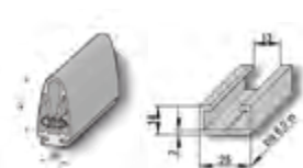
Banda Resistiva SECUBAND 45 SECUBAND 45 resistive band Bande résistive SECUBAND 45 Banda Resistiva SECUBAND 45
